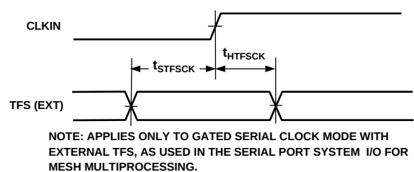
Figure 22. Serial Ports
