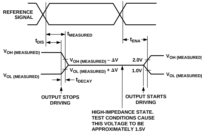
Figure 25. Output Enable/Disable
